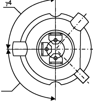
PU43t-4
