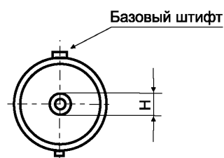
BA20s
