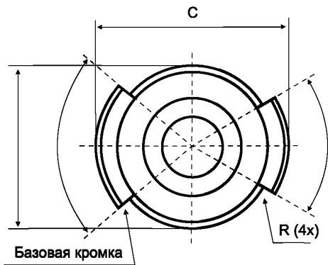
P28s/24
