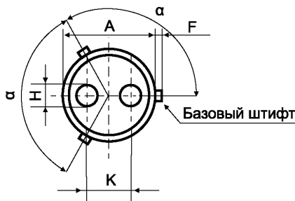
BA21d
