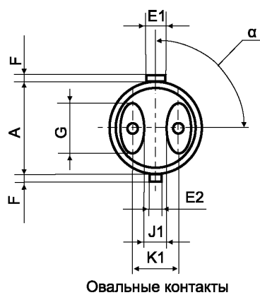
BA20d
